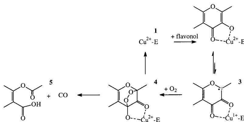
FIGURE 5: Schematic representation of a possible mechanism of 2,3QD-mediated dioxygenation of flavonols as derived from model studies on copper flavonolate-catalyzed dioxygenation of 3-hydroxy flavone (15).
